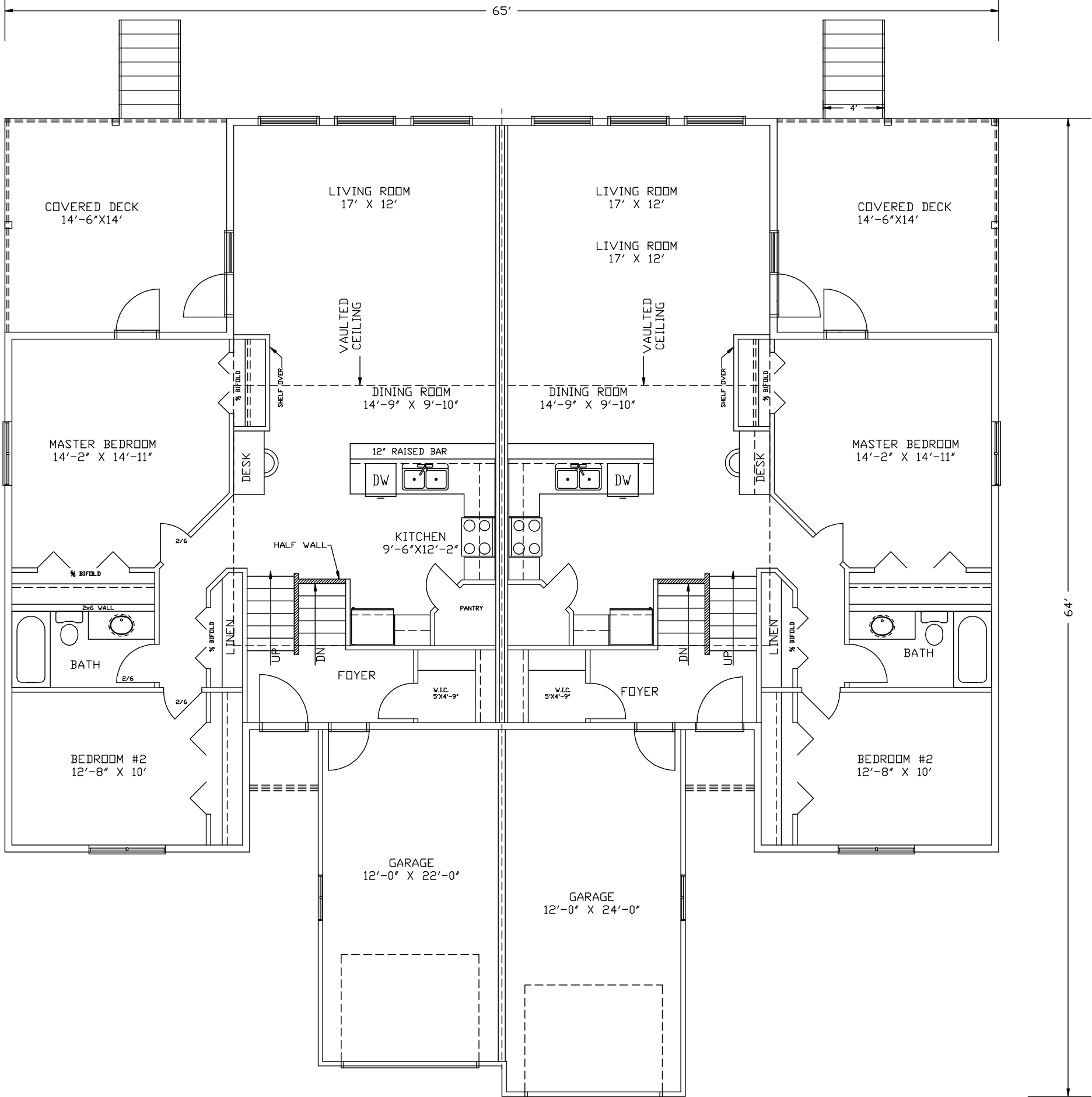
MAIN FLOOR PLAN 1225 sf
