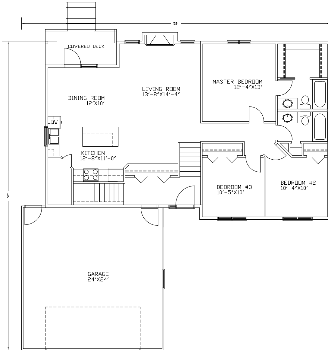
MAIN FLOOR PLAN 1349 SF
