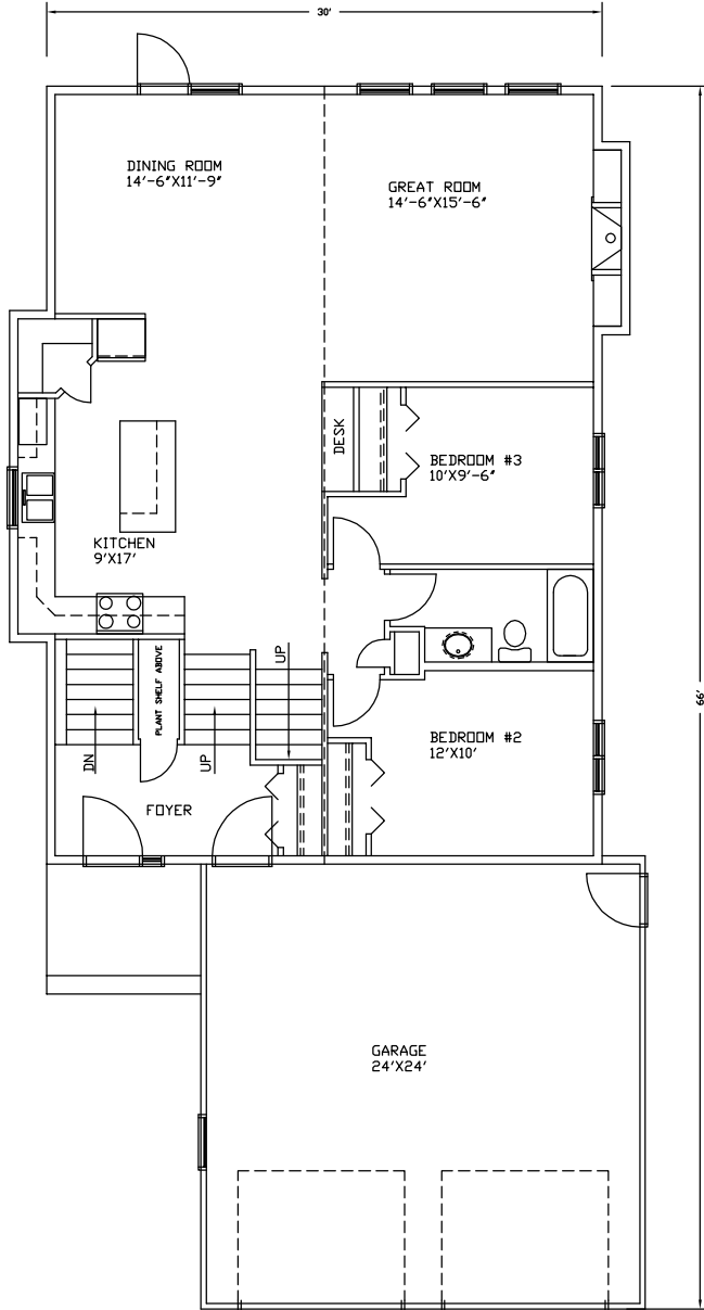
MAIN FLOOR PLAN 1312 SF TOTAL-1719 SF
