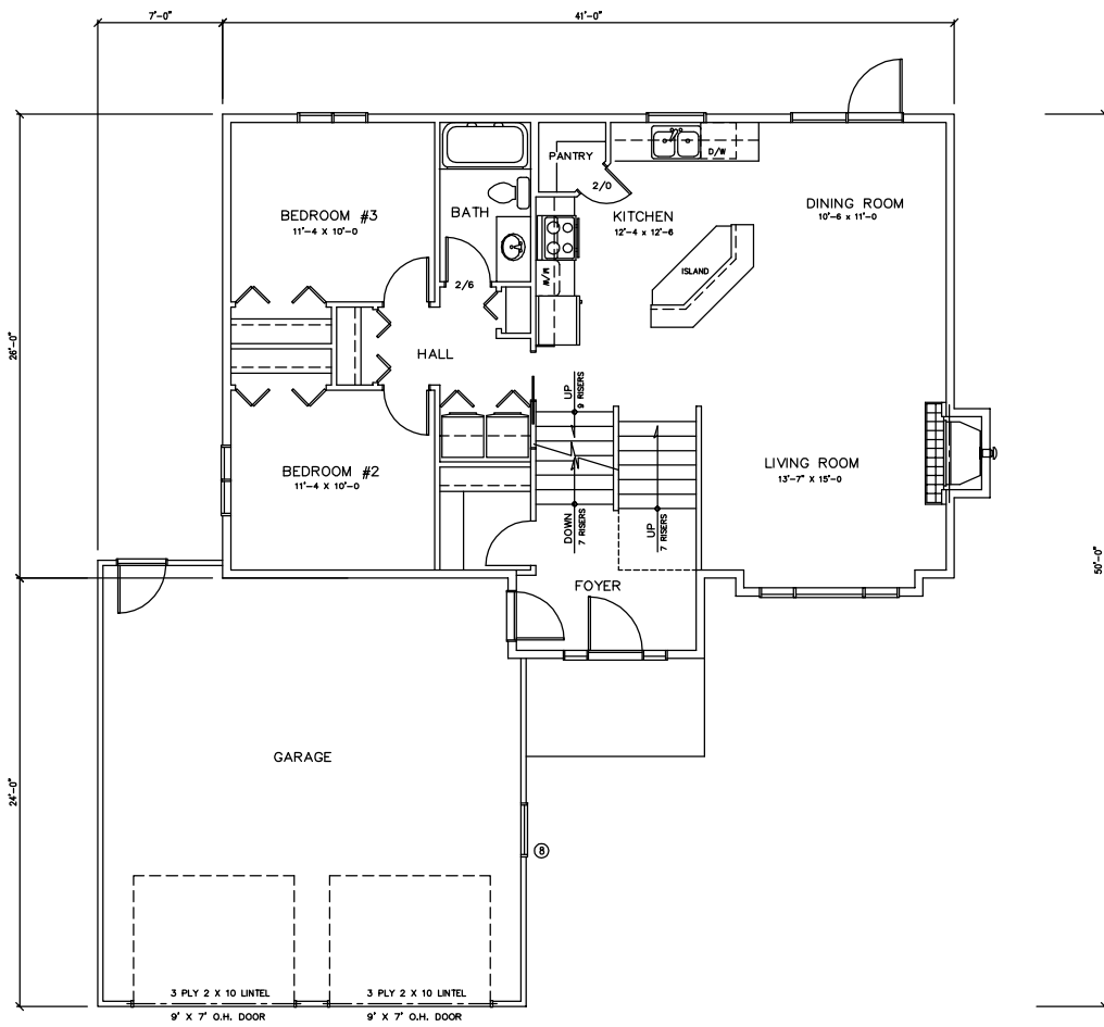
1 MAIN FLOOR PLAN 1136 SQ. FT. SCALE: 1/4" = 1'-0"
