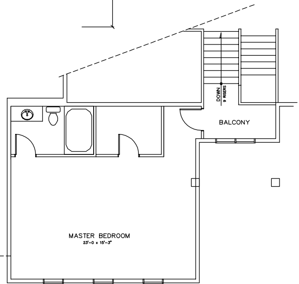
1 SECOND FLOOR PLAN 602 SQ. FT. SCALE: 1/4" = 1'-0"
