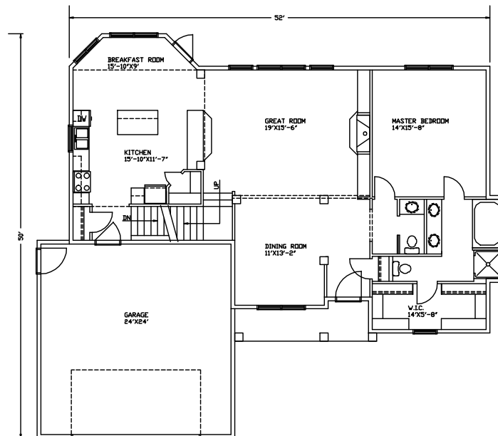
MAIN FLOOR PLAN 1510 SF TOTAL 2600 SF
